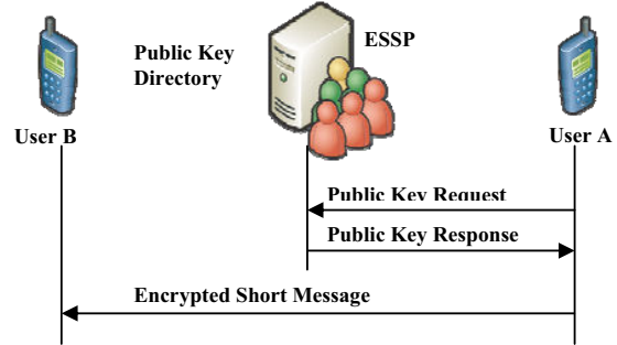
Fig. 3. The RSA procedure for sending an encrypted short message
